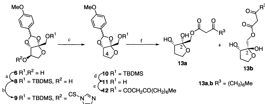
Scheme 3. Synthesis of the 4-deoxy-D-xylulose- \beta -ketodecanoate 13 . Reagents and conditions: (a) TBDMSCl, pyridine, 72%; (b) TCDI, DMAP, THF, 92%; (c) \text{Bu}_3\text{SnH} , toluene, \Delta , 72%; (d) TBAF, THF, 90%; (e) octanoyl-Meldrum's acid, THF, 84%; (f) \text{Pd}(\text{OH})_2/\text{C} , AcOH, 62%.
